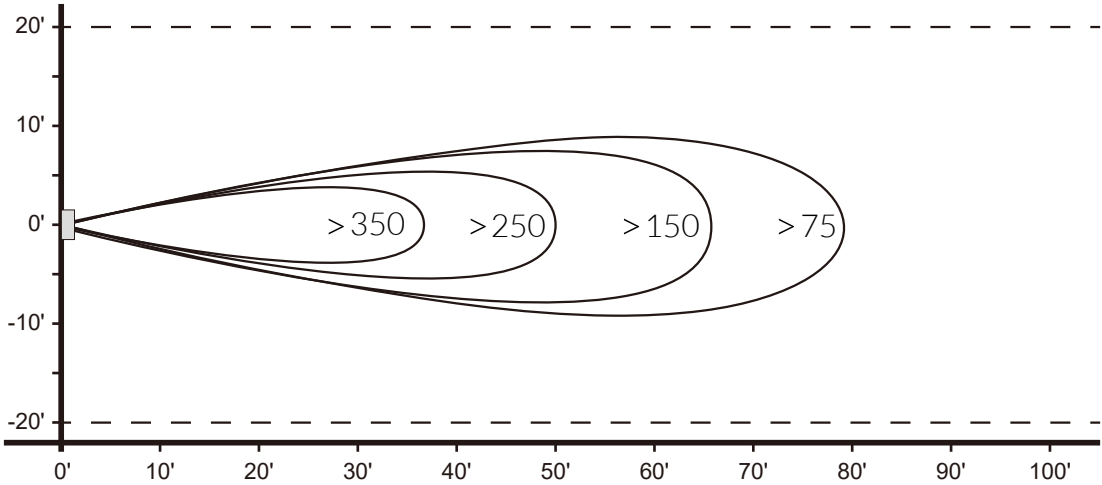
AIR FLOW PATTERN (FULL SPEED)
