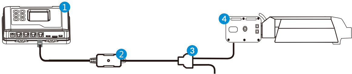
1. Controller 2. Lighting Control Adapter S 3. Splitter 4. P Ballast
