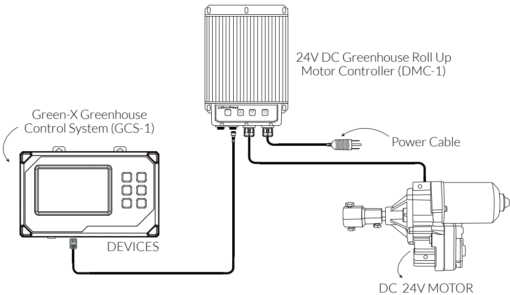
CONNECTION DIAGRAM
